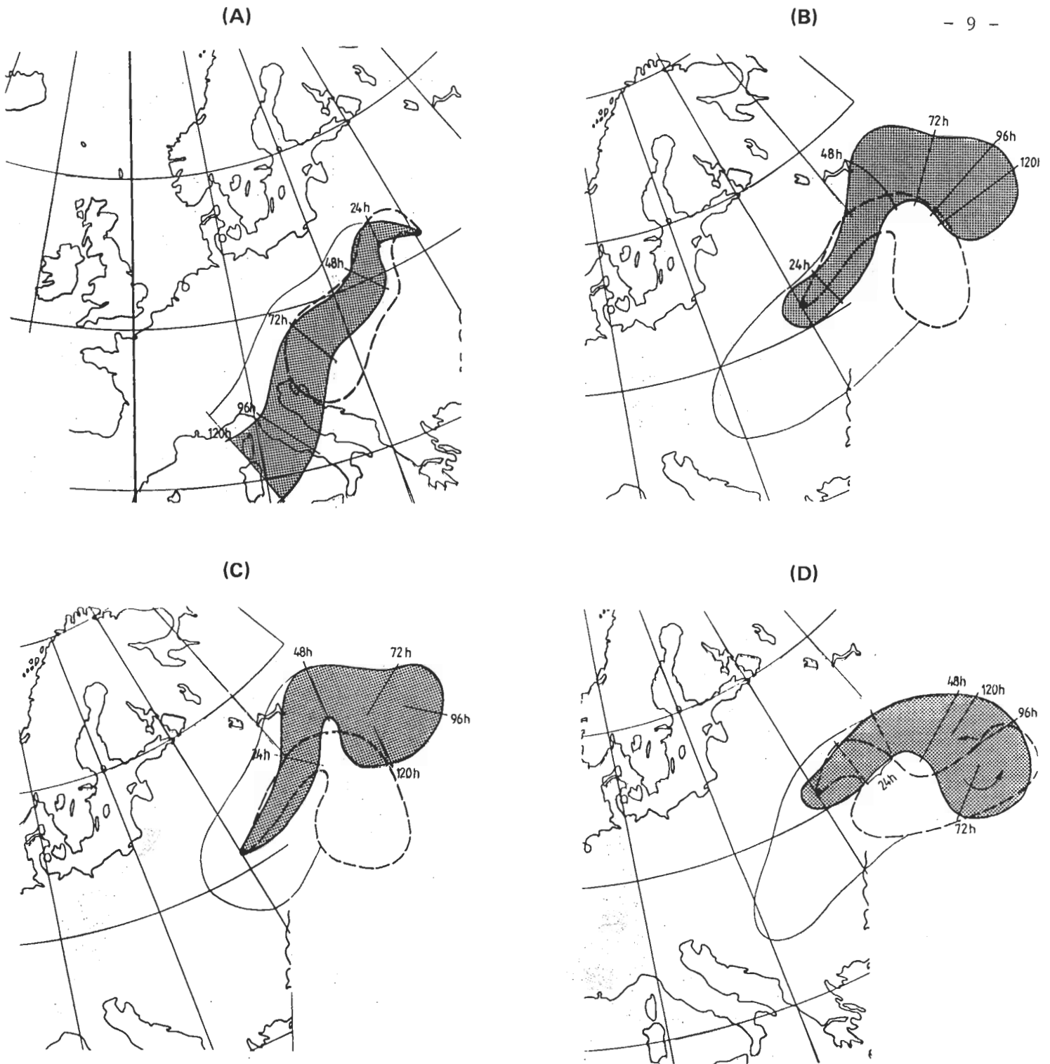
Figures 4 a, b, c and d illustrate the movement in the atmosphere of any radioactive material that might have been released from the Chernobyl reactor during the period Sunday, 27 April to Tuesday, 29 April. The notations are the same as in Figure 3, with the transport times given for the level 1500 m. The four diagrams represent the following emission times at Chernobyl:
